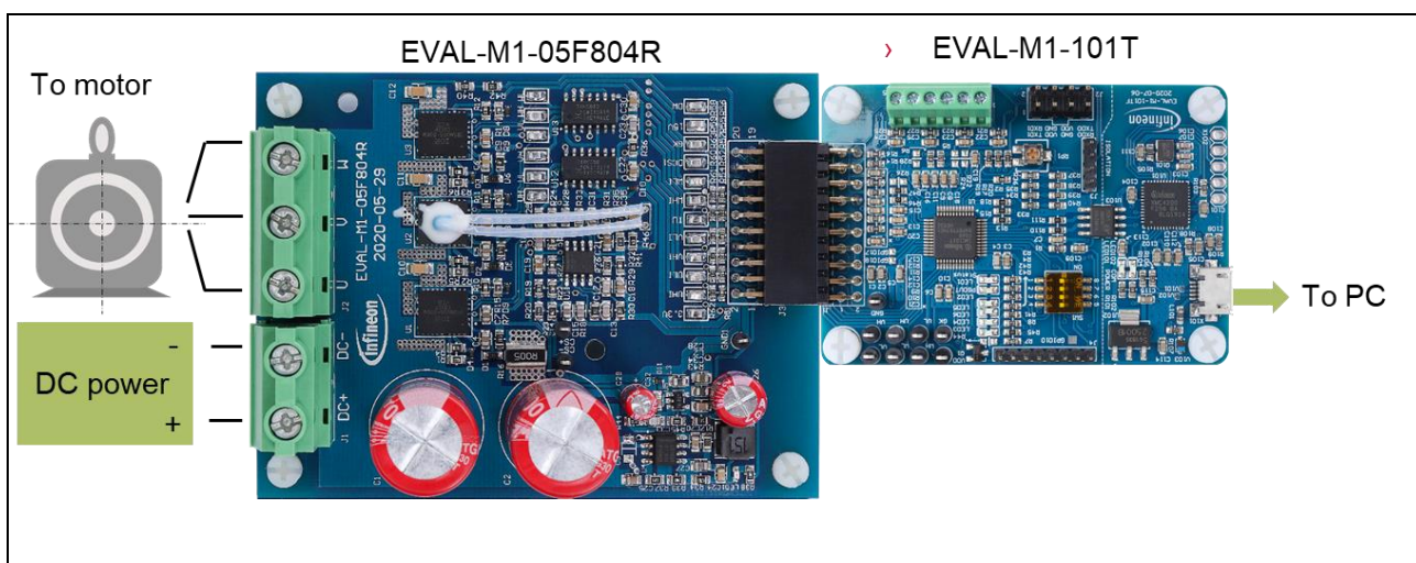
Figure 5 System connection example using EVAL-M1-101T and EVAL-M1-05F804R
