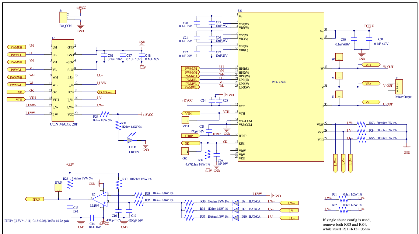
Figure 24 Inverter Section Schematics for EVAL-M1-CTE620N3
