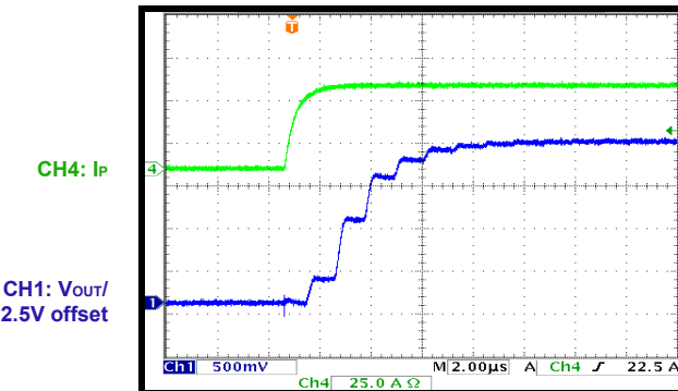
Step-Up Current
