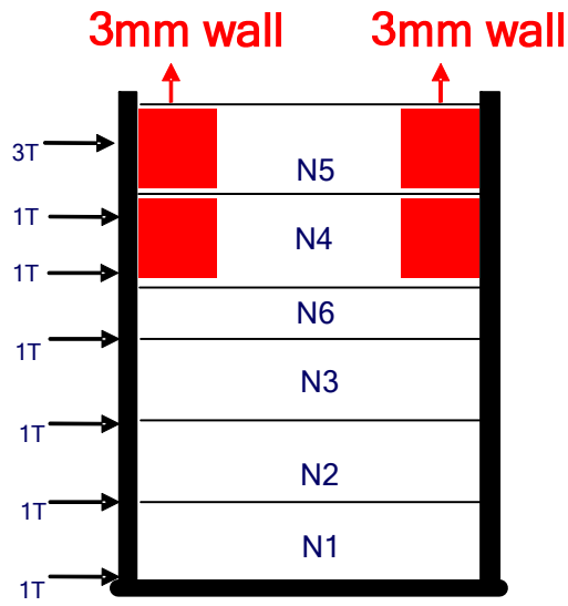
Figure 5—Winding Diagram
