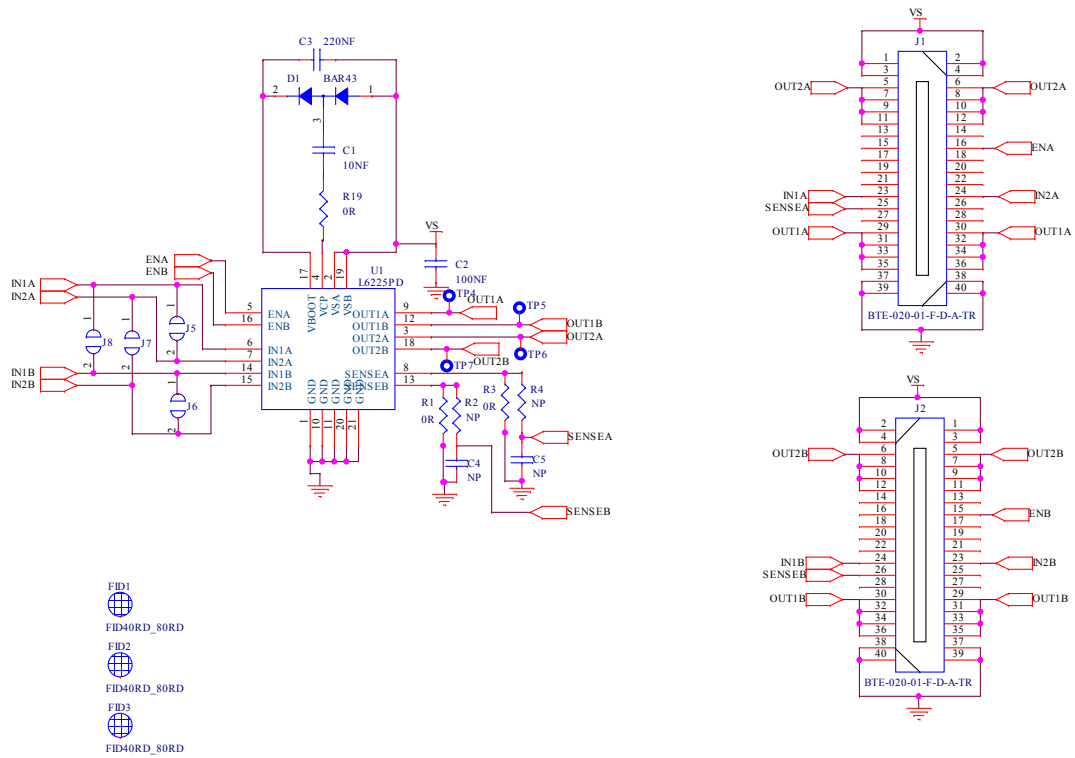
Figure 6. EVL6225-PLUG
