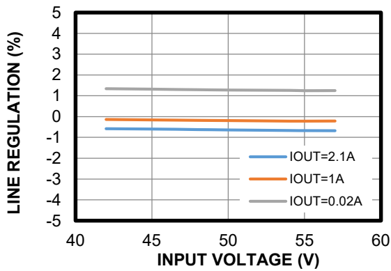
Line Regulation
