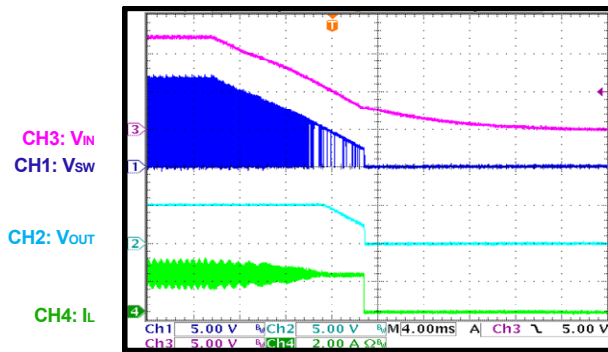
Shutdown I_{OUT} = 2A
