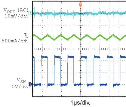
Output Ripple Voltage I_{OUT} = 2A
