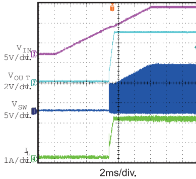
Power On I_{OUT} = 2A
