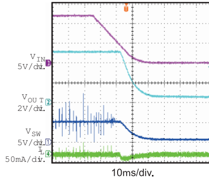
Power Off I_{OUT} = 0A
