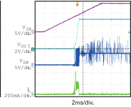
Power On I_{OUT} = 0A
