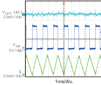
Output Ripple Voltage I_{OUT} = 0.1A
