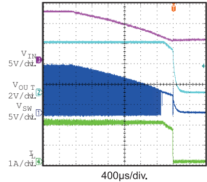
Power Off I_{OUT} = 2A
