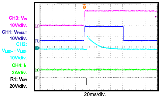
PWM Dimming LED open, start-up through VIN
