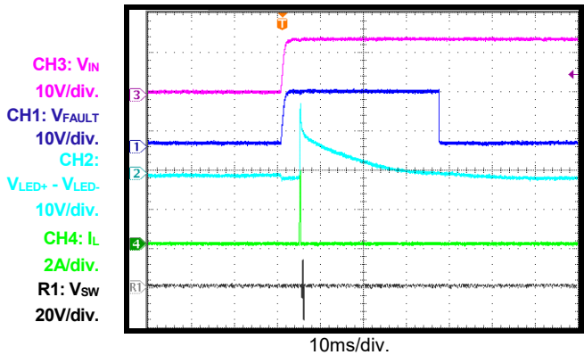
Two-Step Dimming LED open, start-up through VIN
