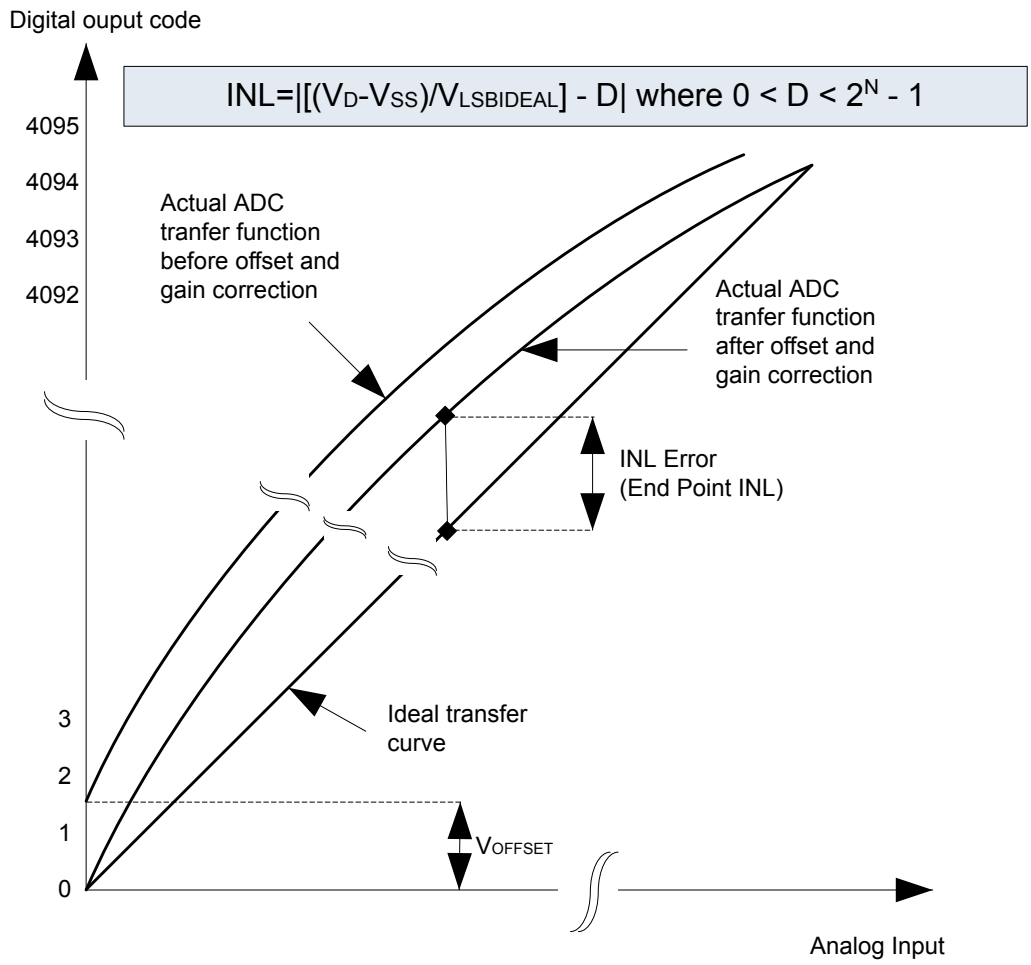
Figure 4.27. Integral Non-Linearity (INL)
