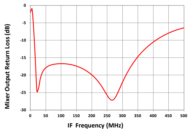
Mixer IF Output Return Loss [ S22_{MIXR\_IF} ]
