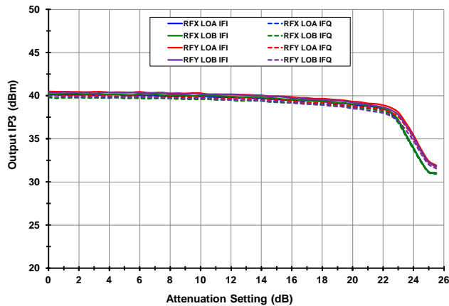
OIP3 [0.8 GHz RF, HiSide Inj.]
