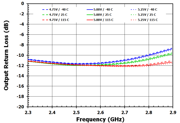
Figure 5. Output Return Loss
