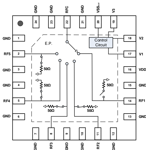
Figure 2. Pin Assignments for 4 x 4 x 0.75 mm 24-QFN – Top View
