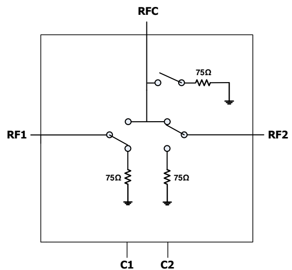
Figure 1. Block Diagram
