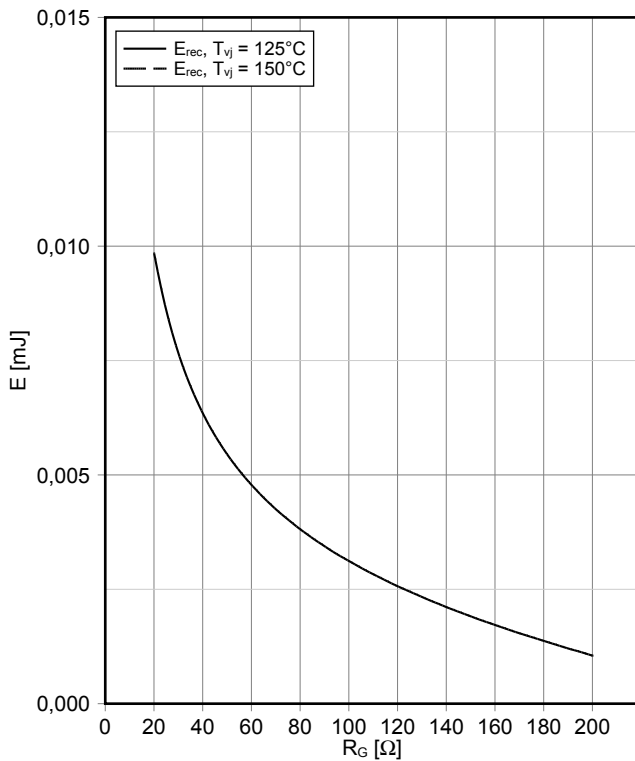
开关损耗 二极管, 三电平 (典型) switching losses Diode, 3-Level (typical) E_{rec} = f(R_G) I_F = 8 A, V_{CE} = 300 V
