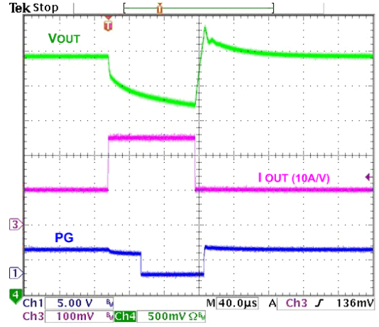
Figure 18. Transient Overload, 1.0–2.5 A, 100 ns Edge
