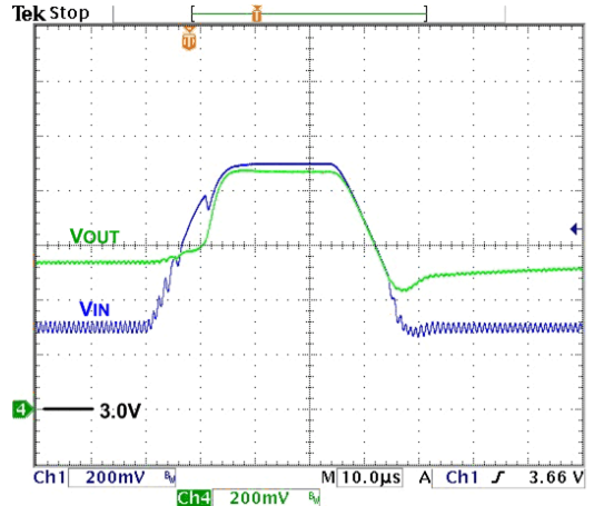
Figure 20. Line Transient, 3.3–3.9 V_{IN} , 10 \mu\text{s} Edge, 1.0 A Load
