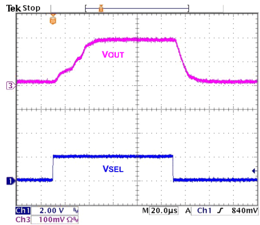
Figure 22. V_{SEL} Step, V_{IN} = 3.0\text{ V} , 500 mA Load
