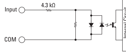
FC4A-M08BR1, FC4A-M24BR2
