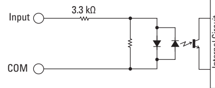
FC4A-N08A11
