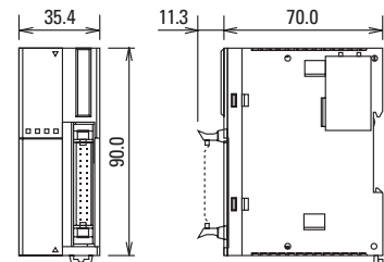
FC4A-D20K3, FC4A-D20S3
