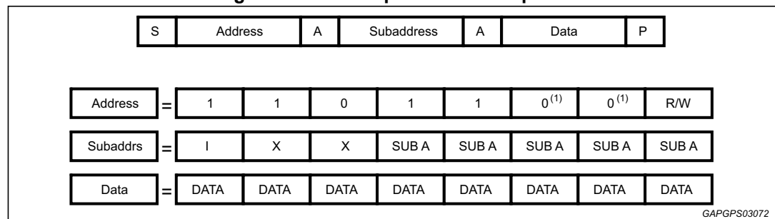
Figure 73. I 2 C bus protocol description
