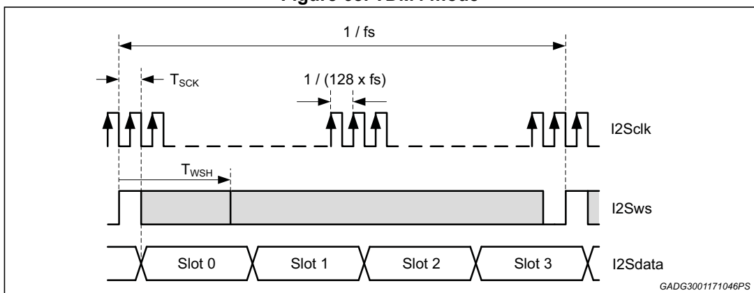
Figure 68. TDM4 mode
