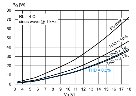
Figure 22. Output power vs. supply voltage ( R_L = 4\ \Omega , sine wave)
