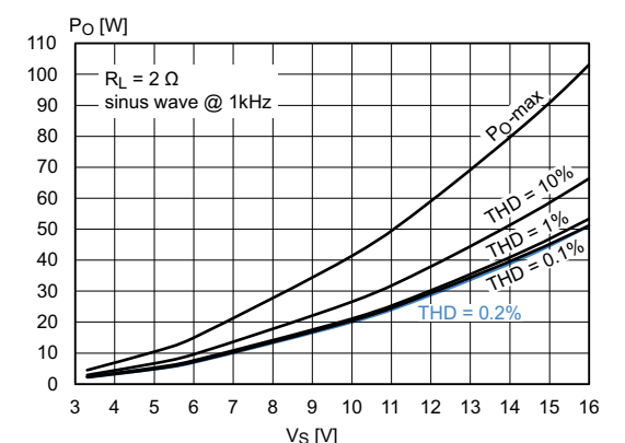
Figure 23. Output power vs. supply voltage ( R_L = 2\ \Omega , sine wave)
