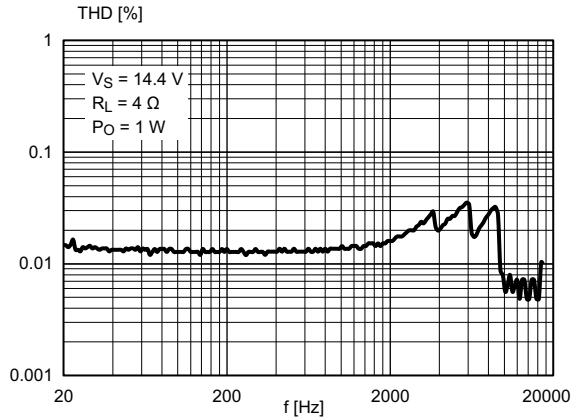
Figure 28. THD vs. frequency ( V_S = 14.4 V , R_L = 4 \Omega , P_O = 1 W )
