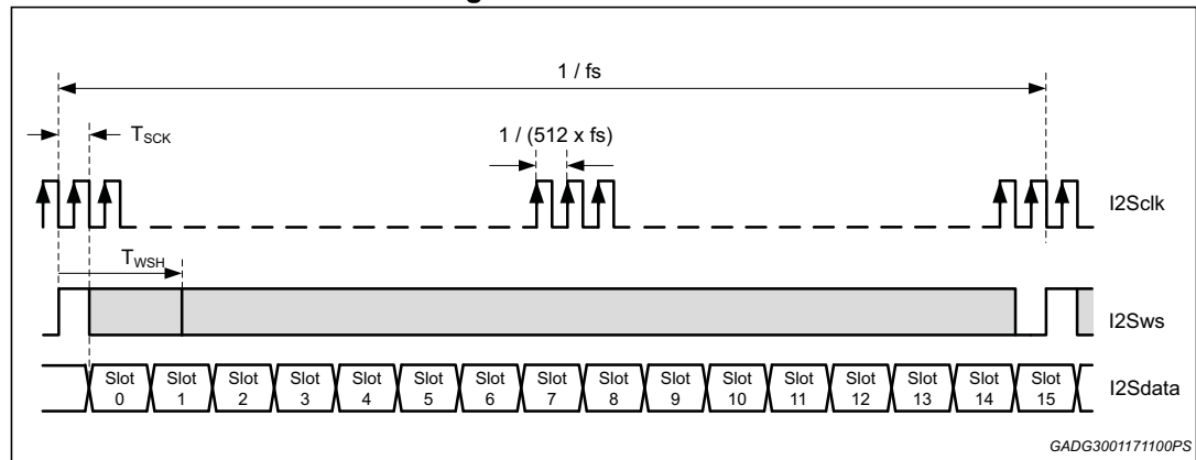
Figure 70. TDM16 mode
