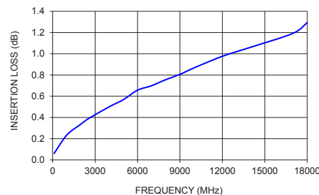
FL141-24SM+ INSERTION LOSS
