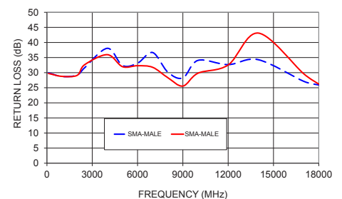
FL141-24SM+ RETURN LOSS
