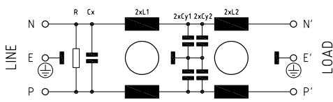
Schematic standard R version (2 to 15A)
