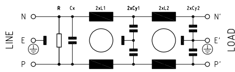
Schematic standard R version (16 to 20A)
