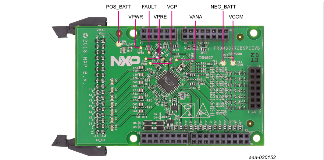
Figure 4. Test points
