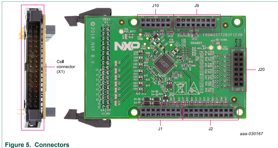
Figure 5. Cell connector (X1)
