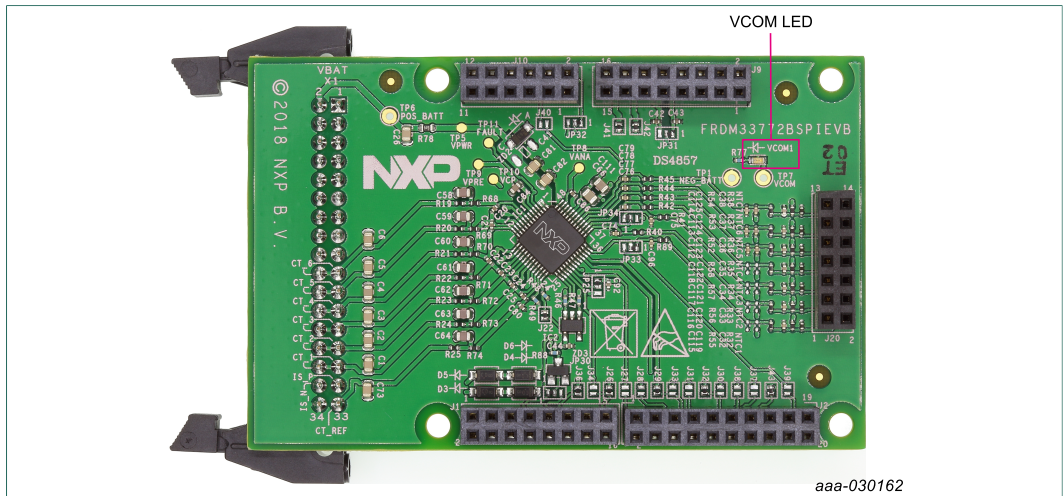
Figure 3. VCOM LED
