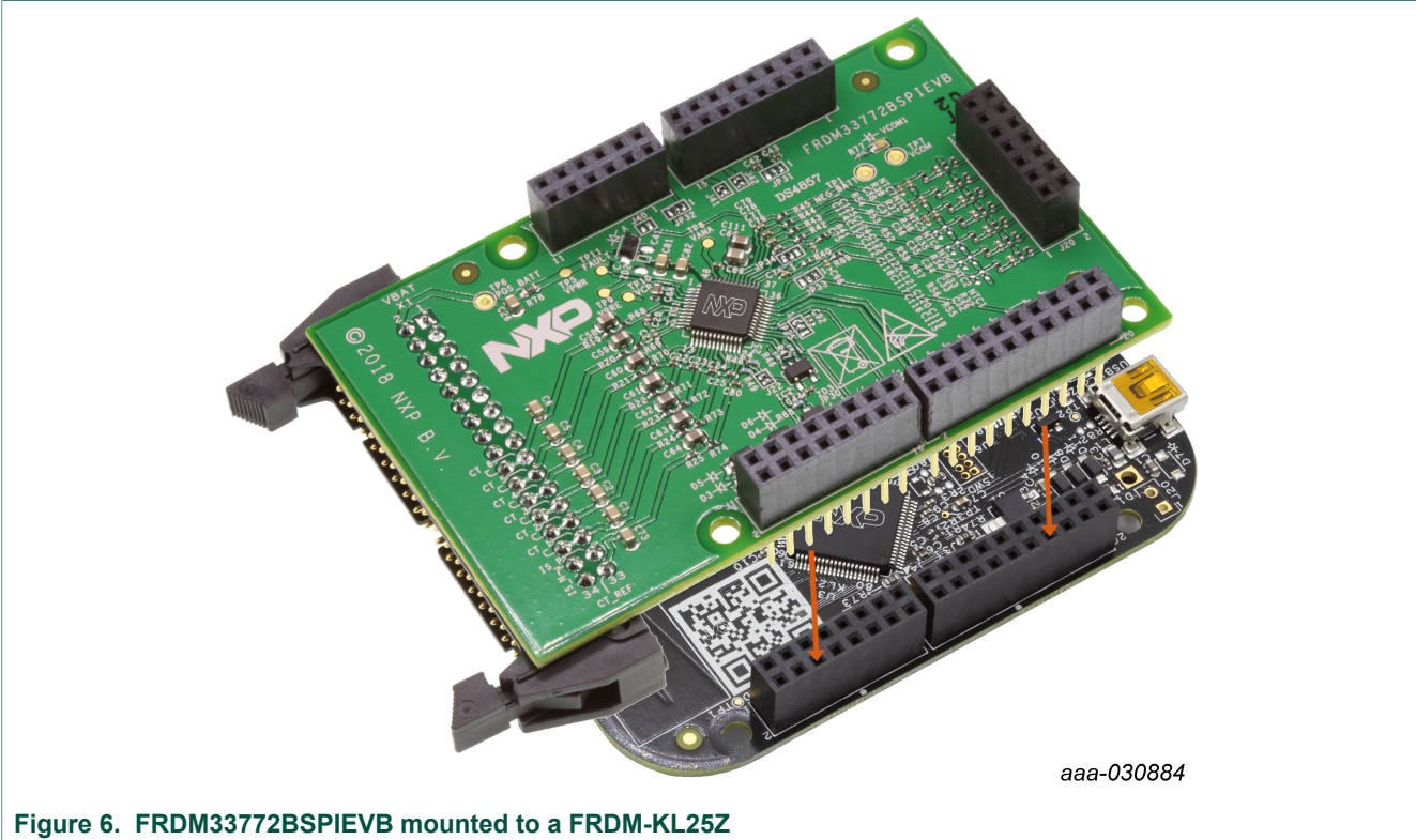
Figure 6. FRDM33772BSPIEVB mounted to a FRDM-KL25Z
