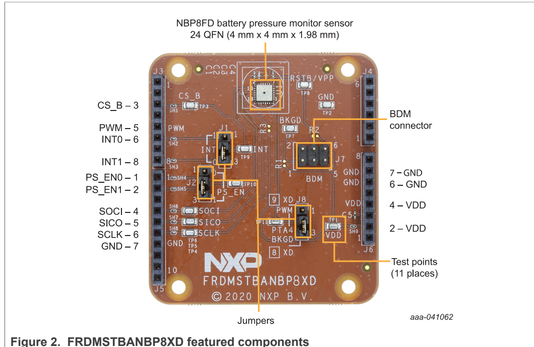
Figure 2. FRDMSTBANBP8XD featured components
