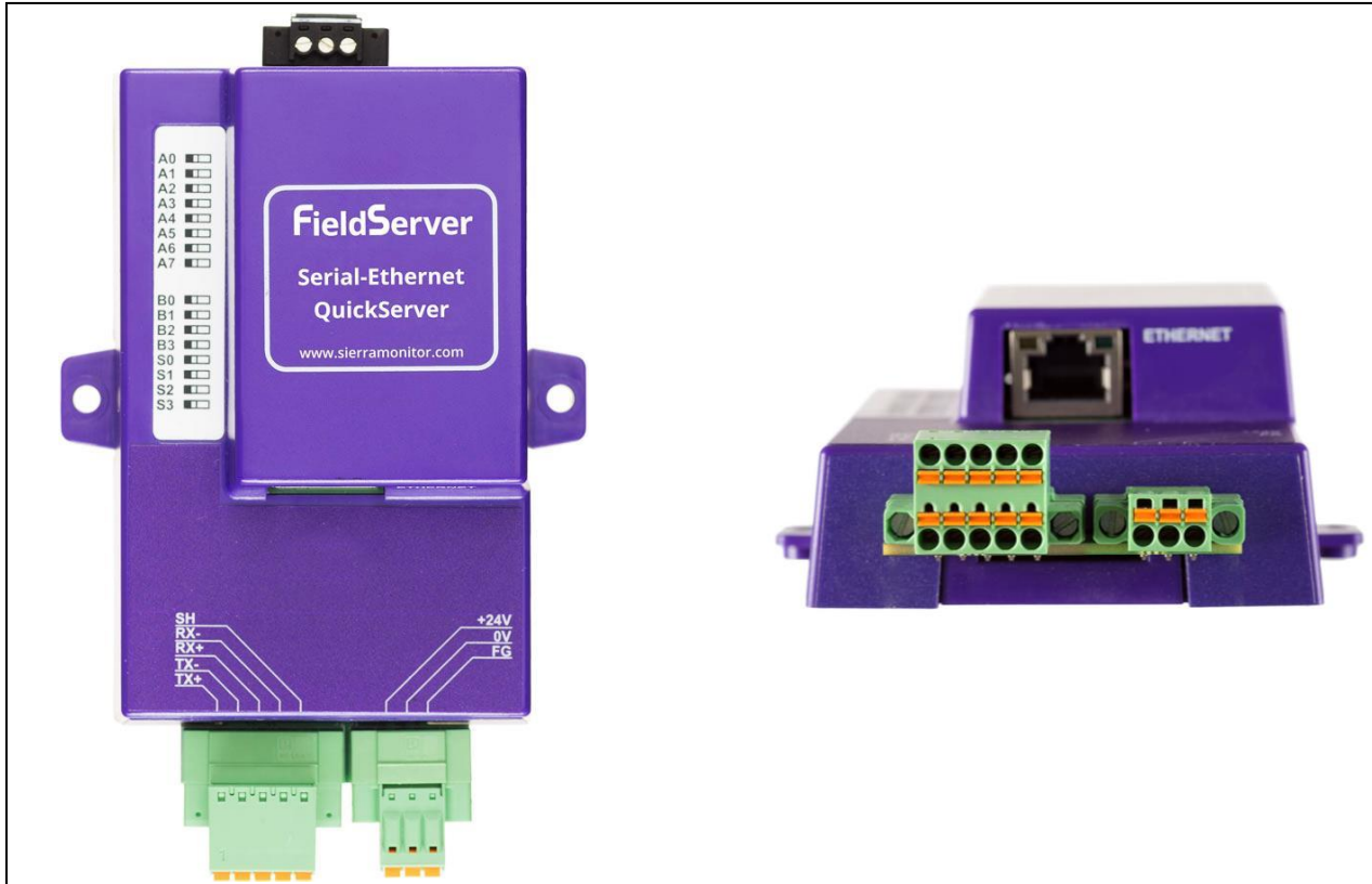
Figure 29: RS-422 Unit
