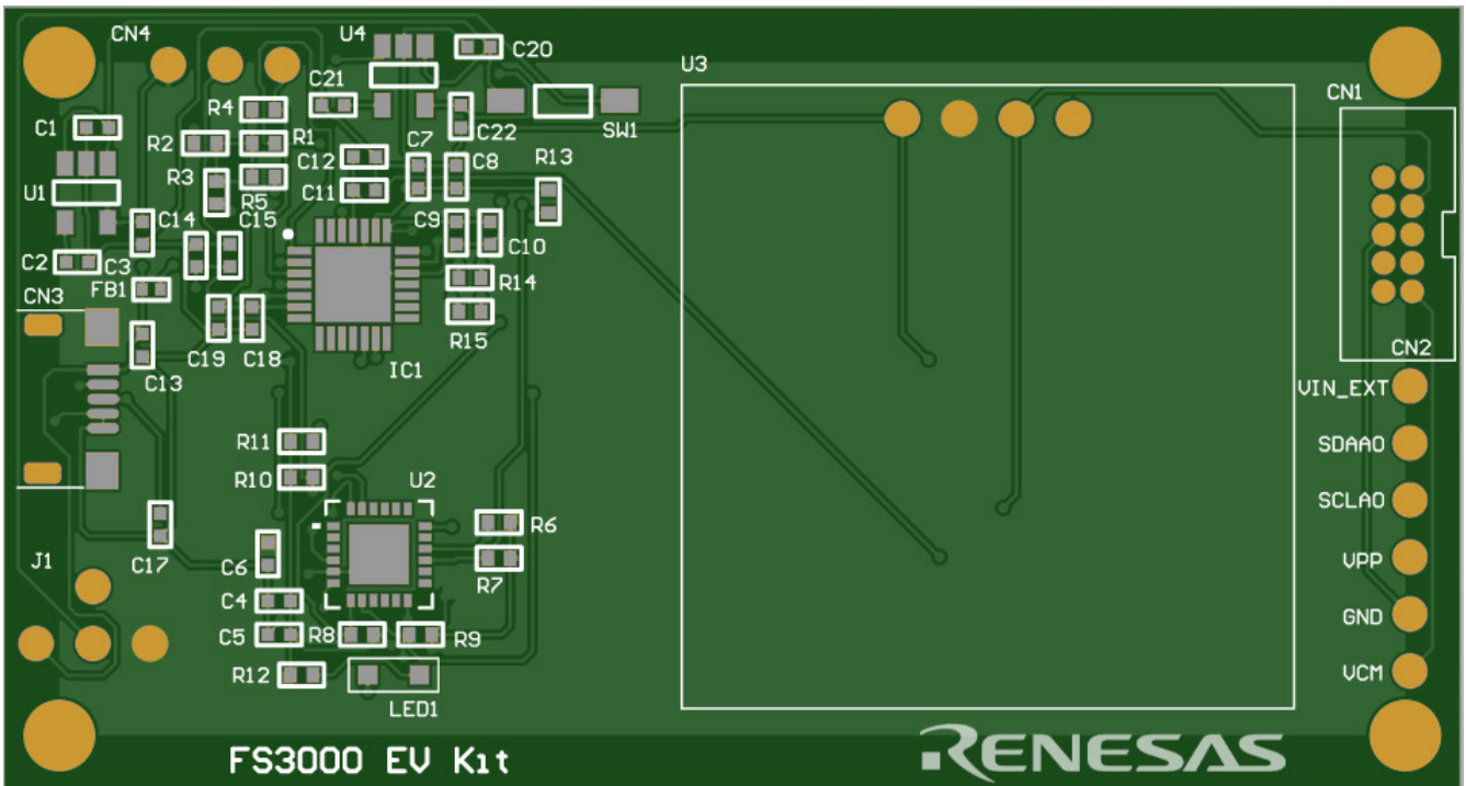
Figure 5. Top Layer
