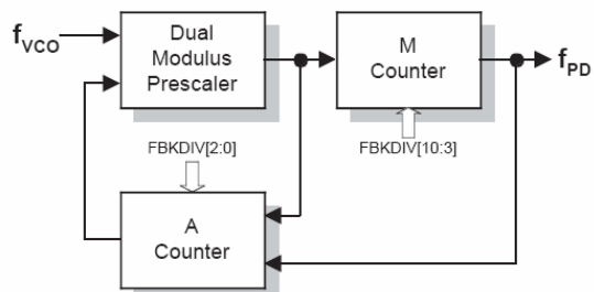
Figure 4. Feedback Divider
