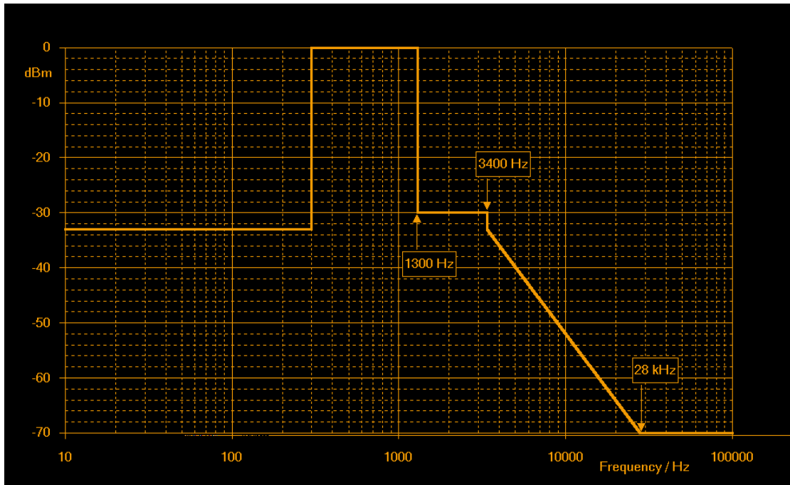
Figure 5a Tx limits at 75bits/sec rate
