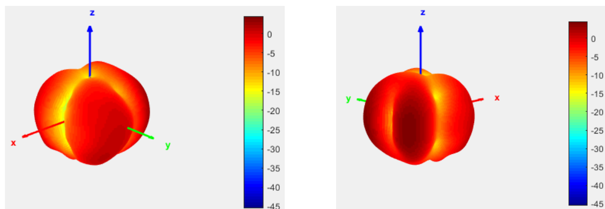
Radiation Pattern at 9GHz
