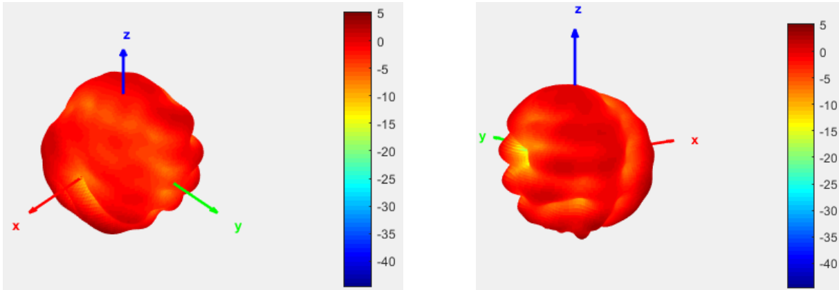
Radiation Pattern at 6.5GHz
