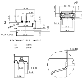
G091131301LF R/A, NORMAL, SMT TYPE
