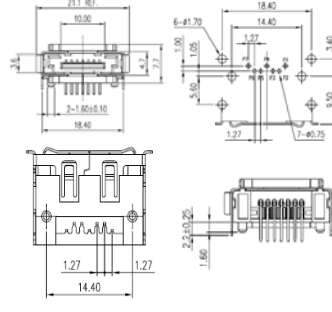
G091172301LF R/A, NORMAL, DIP TYPE
