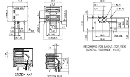
G0925X2301TEU R/A, 2 LAYERS, DIP
