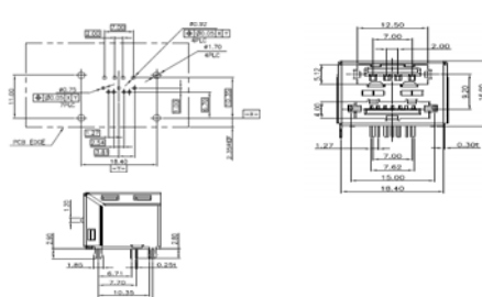
G0927923010ZR USB+ESATA, DIP
