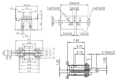
G091352331EU STRAIGHT, DIP
