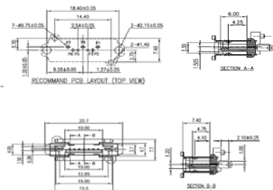
G091351331EU STRAIGHT, SMT
