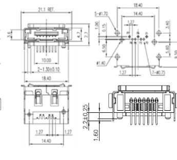
G091282301LF R/A, REVERSE, DIP TYPE
