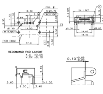
G091231301LF R/A, REVERSE, SMT TYPE
