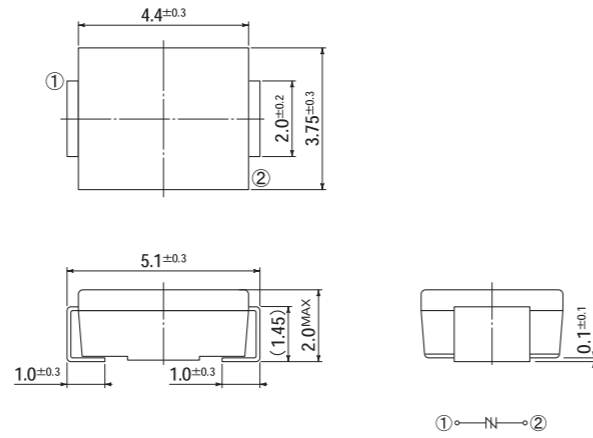
B7 Package: DO-214AA similar M2F
