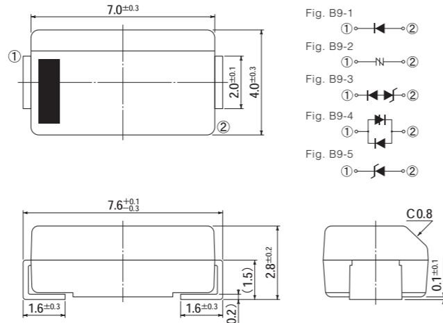
B9 Package: 2F
