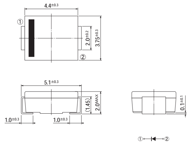
B6 Package: DO-214AA similar M2F
