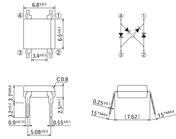
C7 Package: 1NA (DIP)
