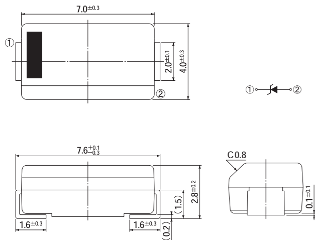
B10 Package: 2F
