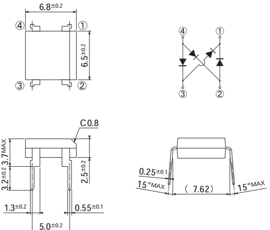
C5 Package: 1N (DIP)
