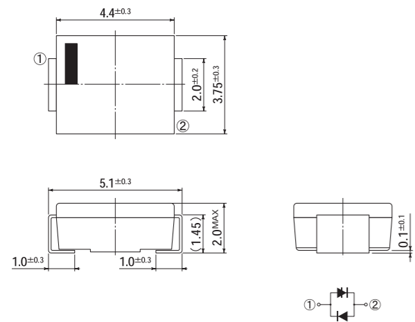
B8 Package: DO-214AA similar M2F
