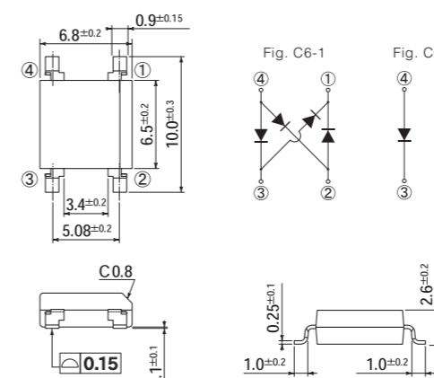
C6 Package: 1NA (SMD)
