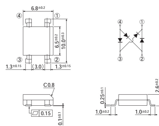
C4 Package: 1N (SMD)
