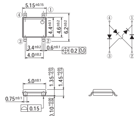
C1 Package: SOPA-4
