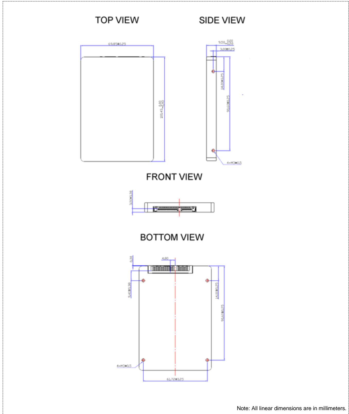
Figure 2-1: SATA 2.5" Industrial Enterprise SSD Dimensions
