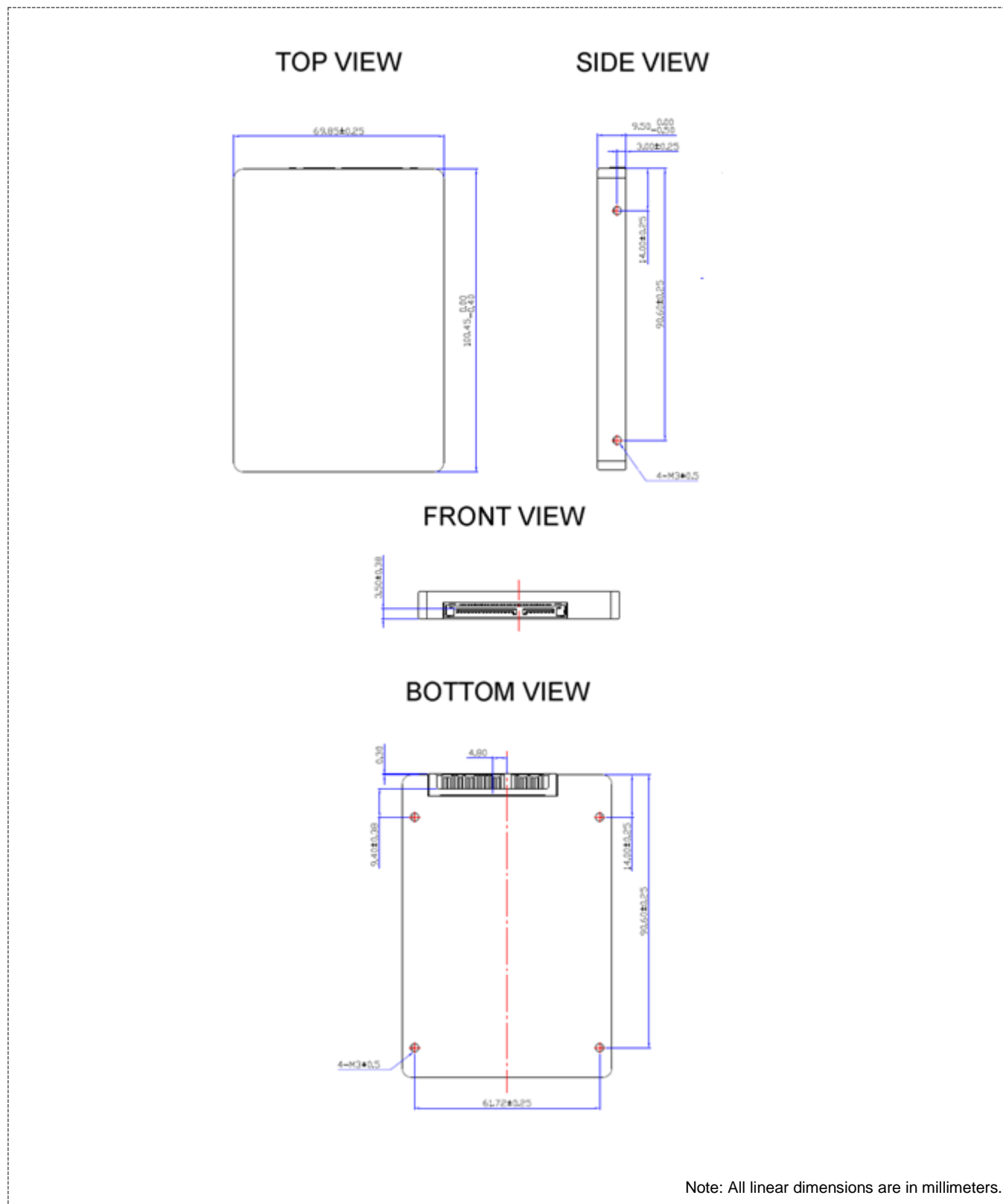
Figure 2-1: SATA 2.5" Industrial Enterprise SSD Dimensions
