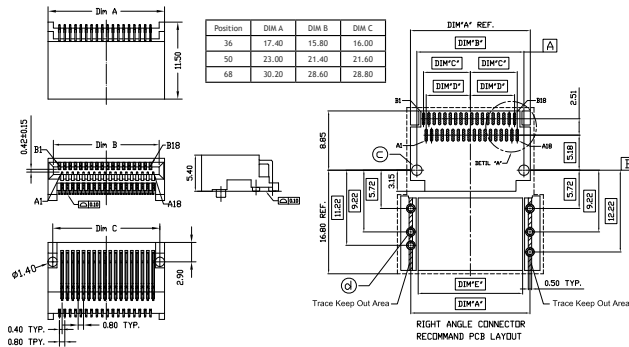
G40BR361BEU
