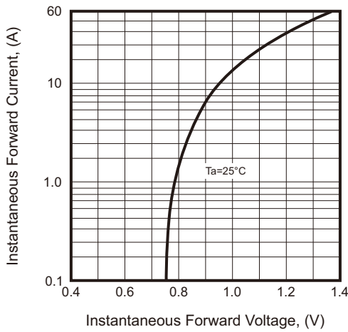
Fig.3 - Forward Voltage
