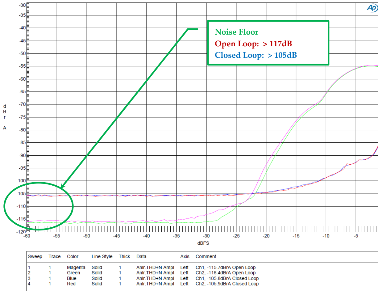
Figure 5. 3 Noise Floor
