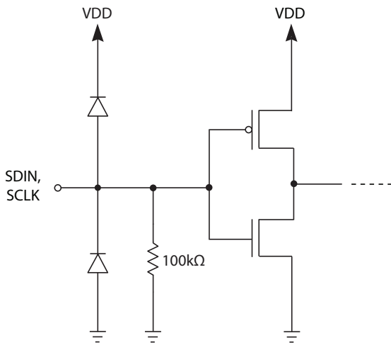
Figure 3-3: SDIN, SCLK
