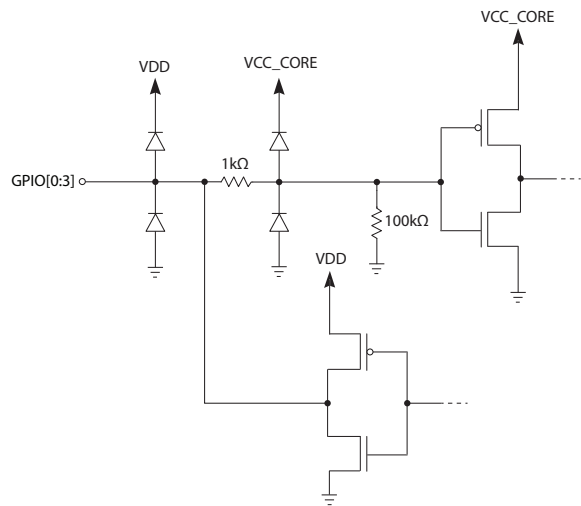
Figure 3-6: GPIO[0:3]
