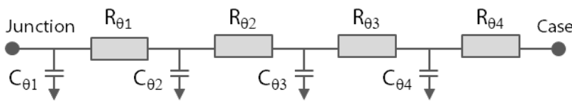
RC breakdown of R_{\theta JC}
