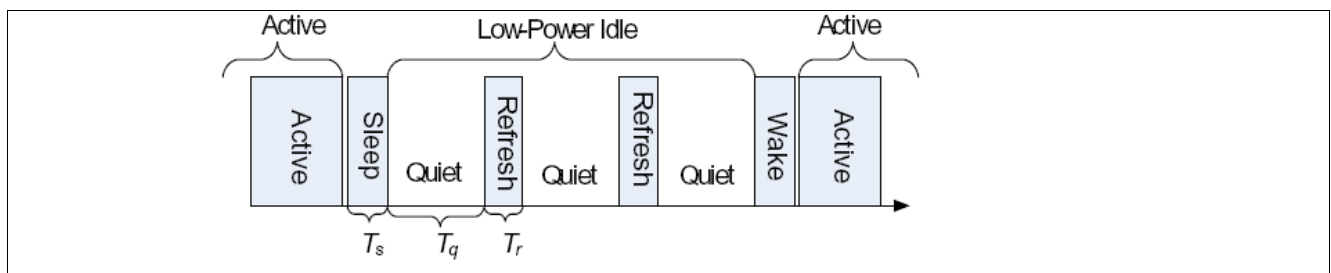
Figure 21 EEE Low-Power Idle Sequence
