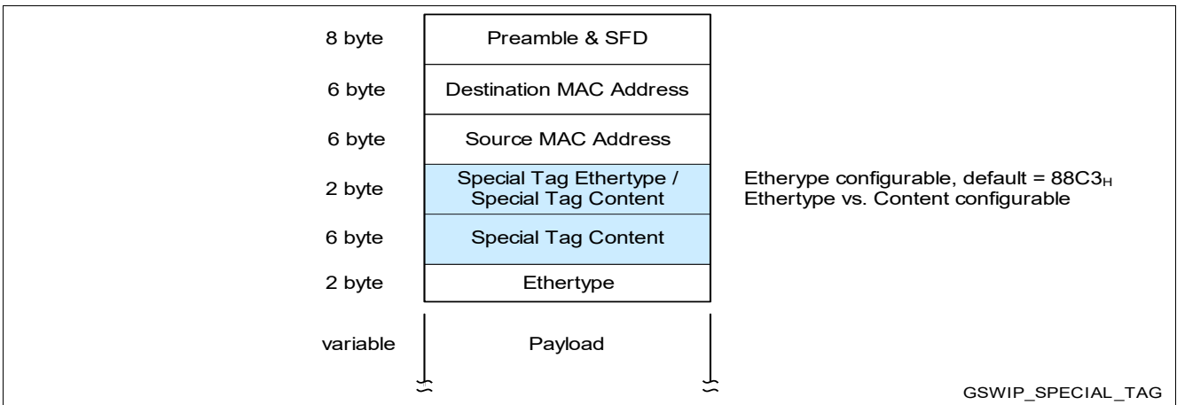
Figure 49 Special tag location in the frame
