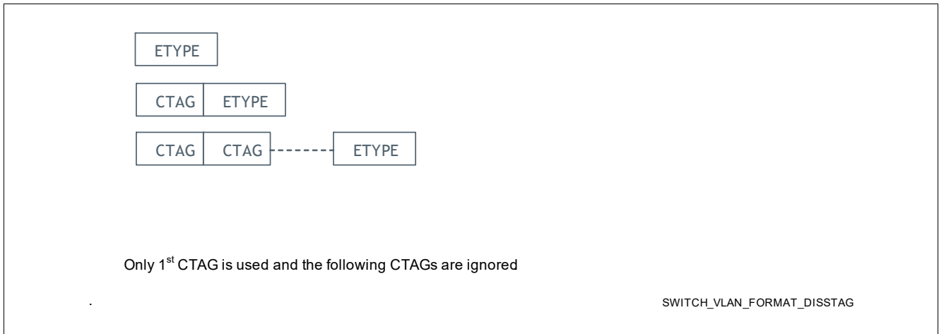
Figure 30 Supported Frame Formats when STAG is disabled
