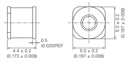
Surface-mount (GTCS25-XXXM-R02)
