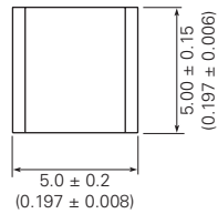
No Leads (GTCN25-XXXM-R02)†
