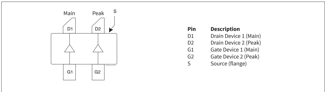
Lead connections for GTRA384802FC
