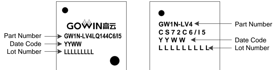
Figure 5-3 Package Mark
