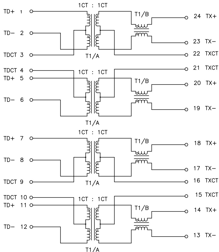
SCHMATIC
