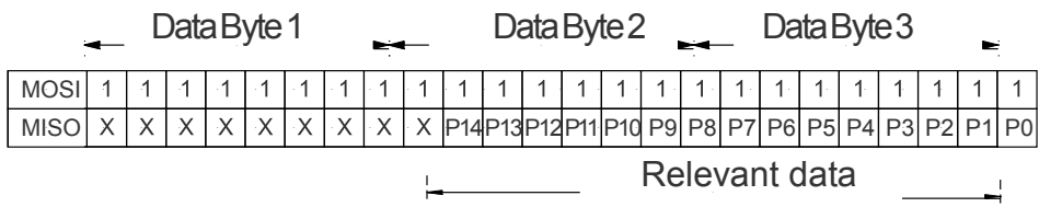
Fig. 2: 3 byte data stream between HCE sensor and master containing the pressure value as a 15 bit information
