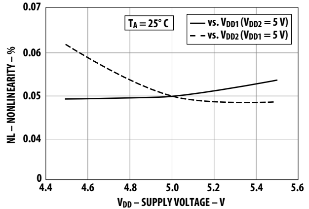
Figure 10 200-mV Nonlinearity vs. V_{DD1} and V_{DD2}
