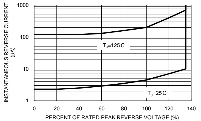
FIG. 2 TYPICAL REVERSE CHARACTERISTICS PER LEG
