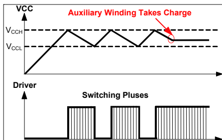
Figure 2: VCC Start-Up
