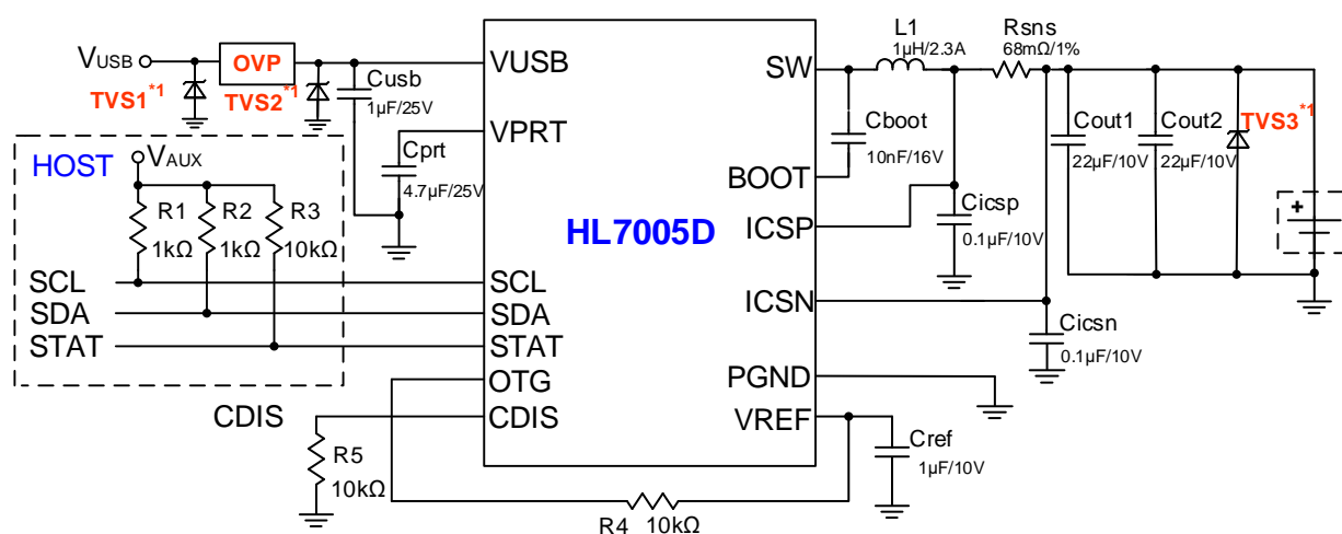
Figure 1. HL7005D Typical Application Diagram
