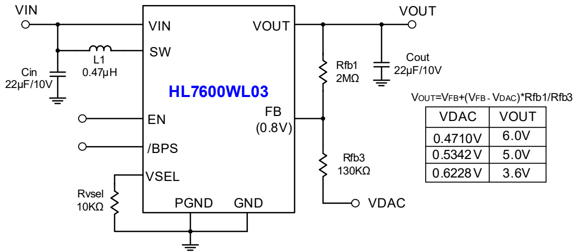
Figure 4 HL7600WL03 Typical Application Diagram, Set V OUT by V DAC
