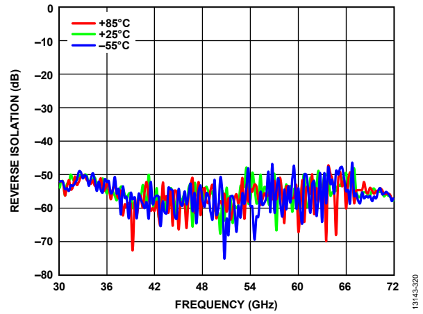
Figure 20. Reverse Isolation vs. Frequency at Various Temperatures
