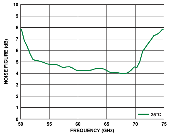
Figure 33. Noise Figure vs. Frequency at 25°C
