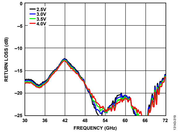
Figure 19. Output Return Loss vs. Frequency for Various V_{DD} at I_{DD} = 250\text{ mA}
