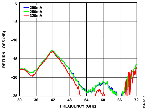
Figure 18. Output Return Loss vs. Frequency for Various I_{DD} at V_{DD} = 4\text{ V}
