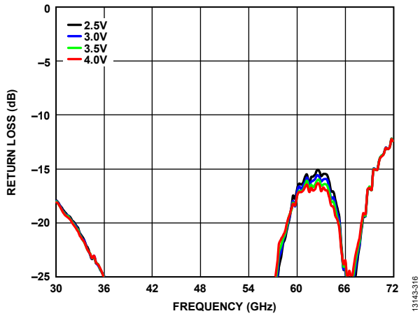
Figure 16. Input Return Loss vs. Frequency for Various V_{DD} at I_{DD} = 250\text{ mA}
