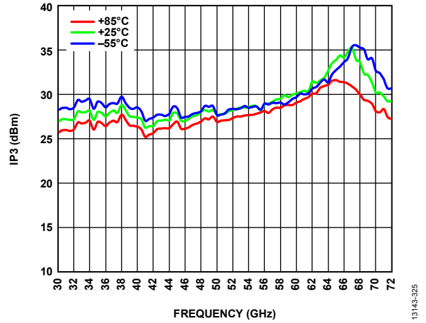
Figure 25. Output IP3 vs. Frequency for Various Temperatures at P_{OUT} = 10 \text{ dBm/Tone}
