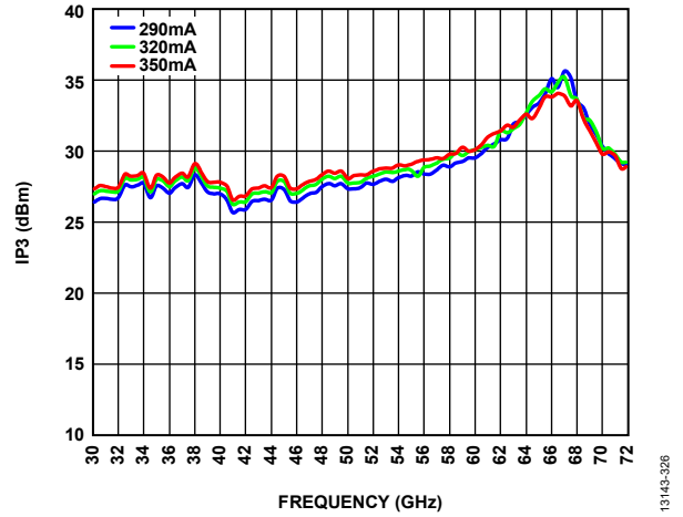
Figure 26. Output IP3 vs. Frequency for Various I_{DD} at P_{OUT} = 10 \text{ dBm/Tone}
